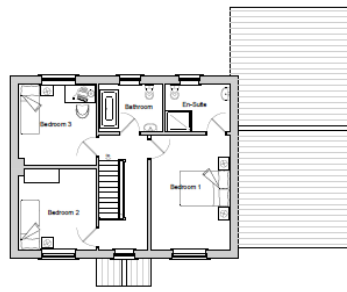
Proposed First Floor
